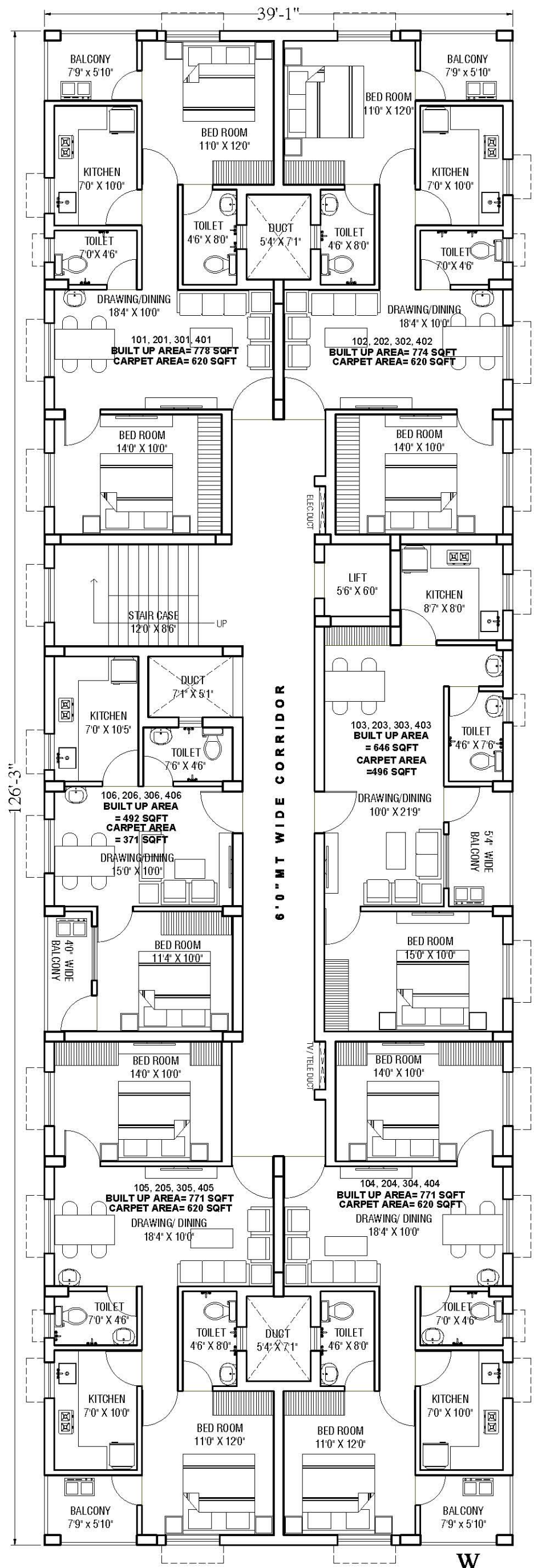
1ST FLOOR PLAN (BLOCK-C)
