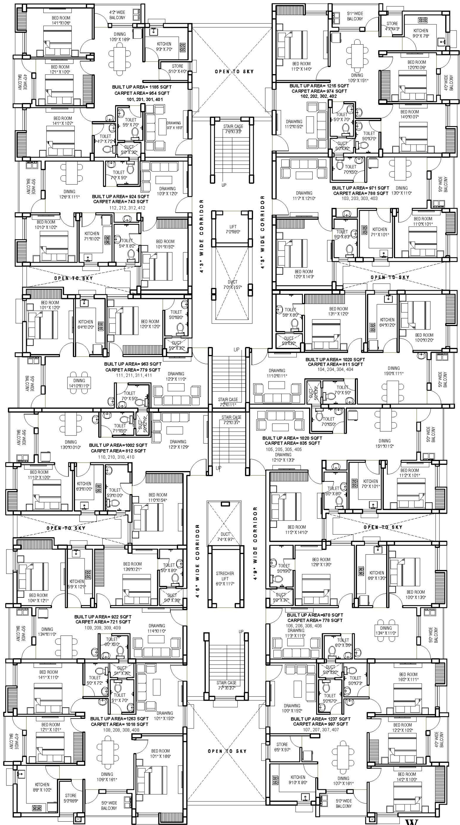
1ST FLOOR PLAN (BLOCK-A)
