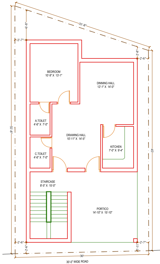
PROPOSED SITE LAYOUT CUM GROUND FLOOR PLAN AREA-1083 SQFT
