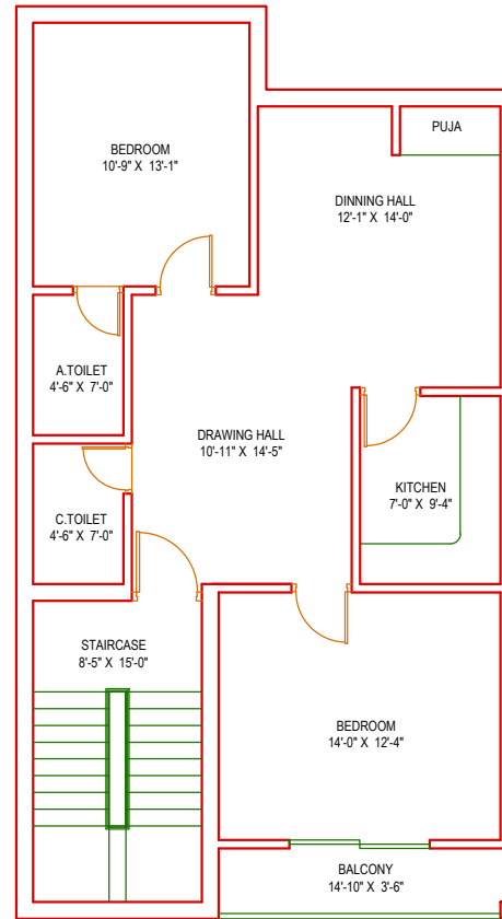
PROPOSED FIRST FLOOR PLAN AREA-1083 SQFT
