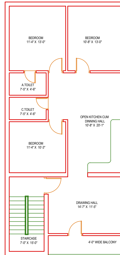
PROPOSED FIRST FLOOR PLAN AREA-1227 SQFT
