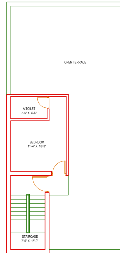
PROPOSED SECOND FLOOR PLAN AREA-360 SQFT
