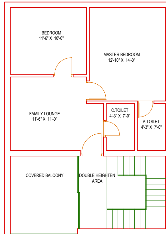
PROPOSED FIRST FLOOR PLAN AREA-871 SQFT
