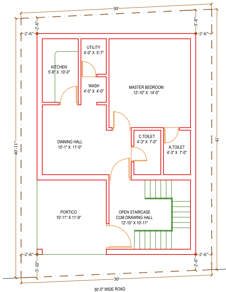
PROPOSED SITE LAYOUT CUM GROUND FLOOR PLAN AREA-871 SQFT
